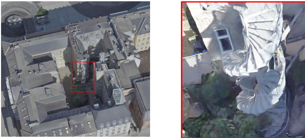
Fig. 6: Problems in the 3D mesh of Copenhagen 2021 become visible at (too) high zoom levels (right)
