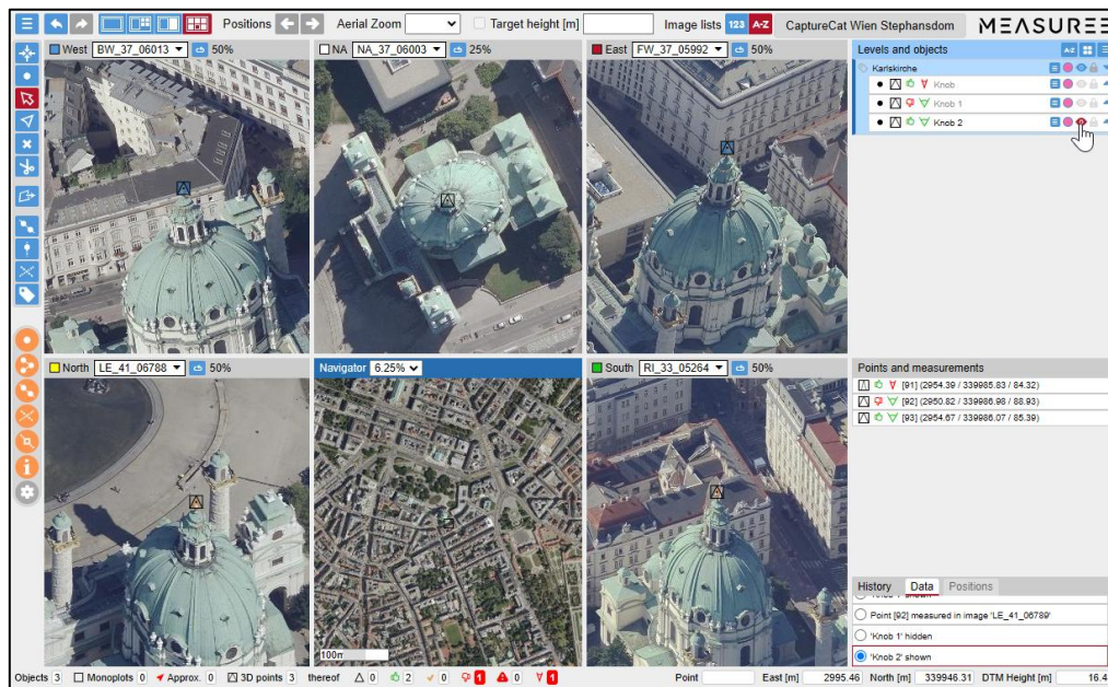
Fig. 43: Knob of the main dome of the Karlskirche Vienna (2020) correctly measured in a nadir image and two oblique images
